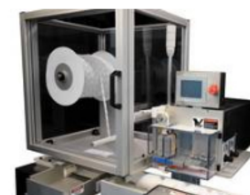
Material Handling & Storage New Pouch Dispenser from AZCO is PLC Controlled
